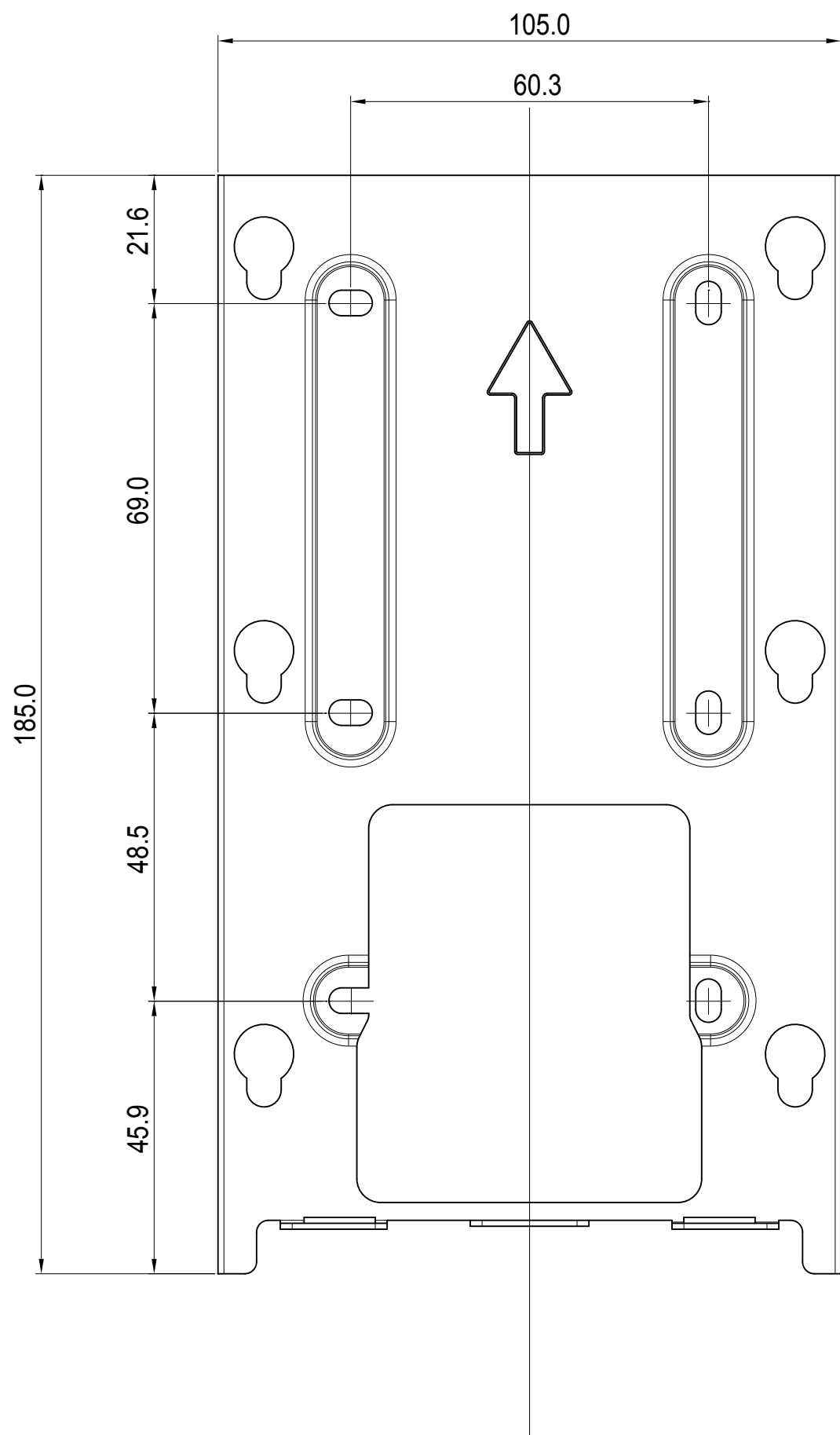
1 FRONT VIEW
