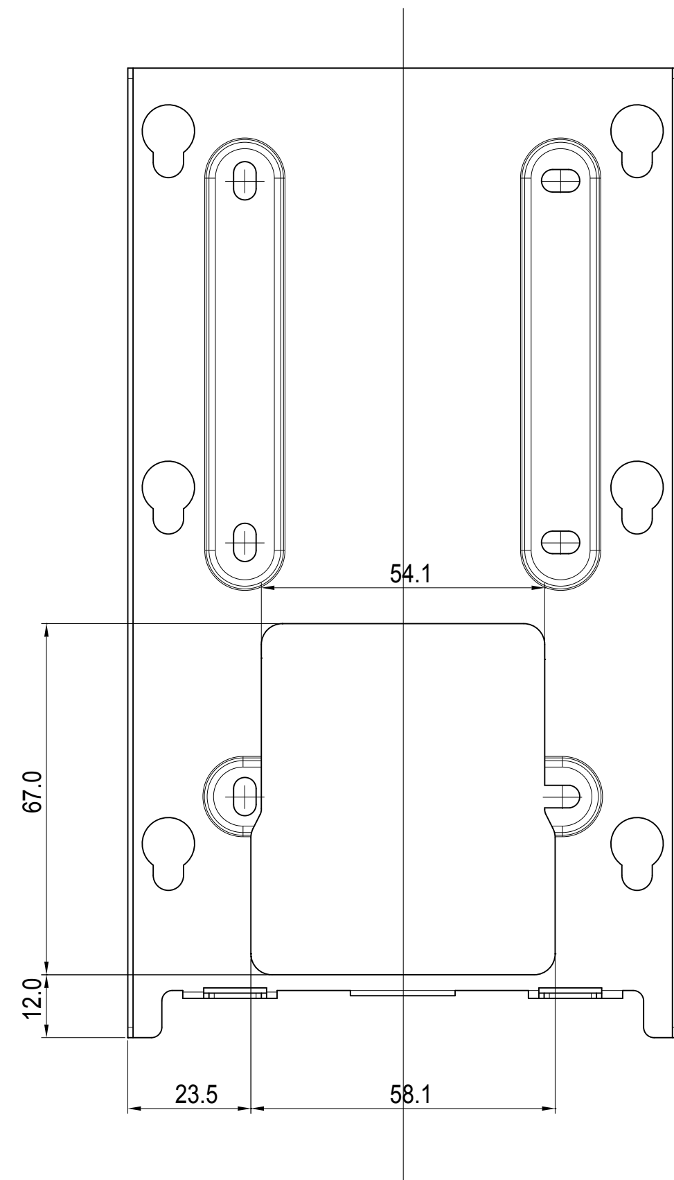
4 BACK VIEW
